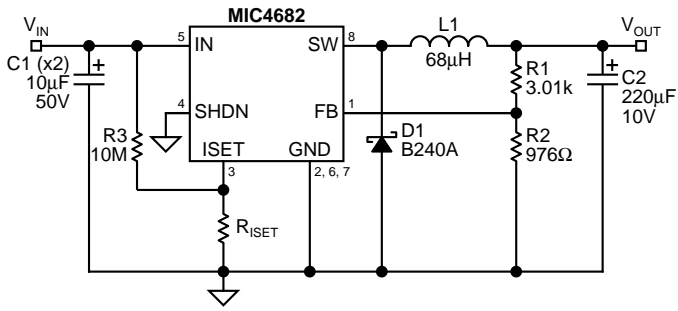
Current Limit Test Circuit
