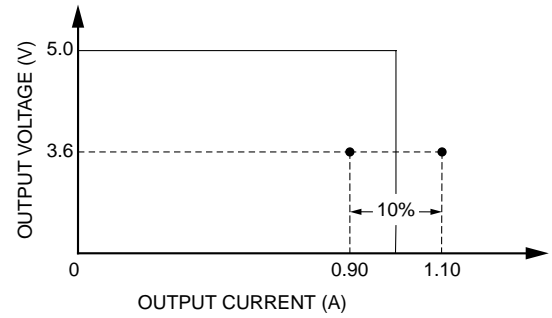
Constant-Current Constant-Voltage Accuracy
