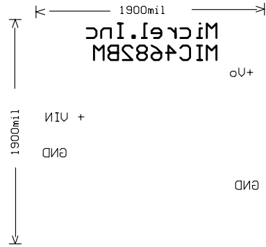
Figure 5d. Bottom Silkscreen
