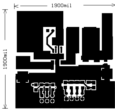
Figure 5c. Top Layer
